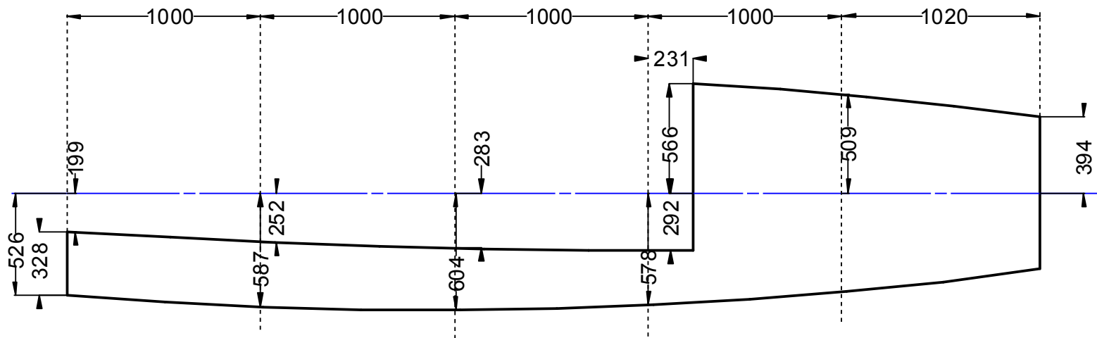
SIDE & AFT DECK (Aft deck covers aft bunk & is cockpit seat.)
